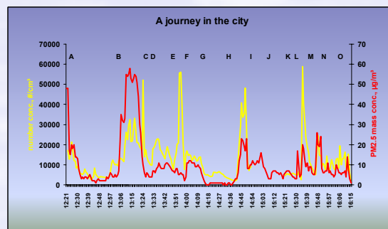
Figure 1. Particle mass (PM 2.5 ) and number (0.02 - > 1 µm) concentrations in different environments A: metro station, AB: commuting in a metro, BC: metro/railway station CD: street, DE: bus1, EF: street, FG: bus2, GH: cafe, HI: railway station, IJ: local train1, JK: station2, KL: train2, LM: train3, MN: railway station, NO: street.
